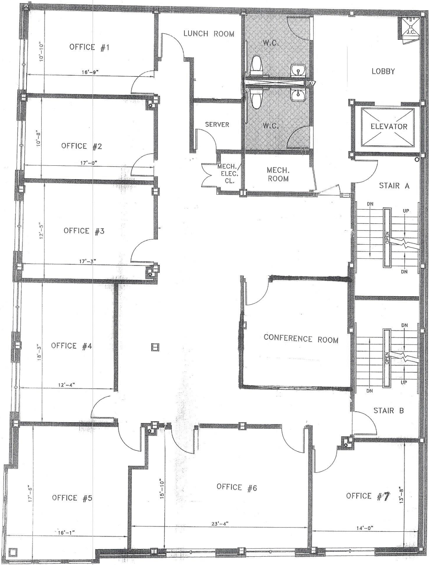
6 5TH FLOOR PLAN SCALE: 1/4" = 1'-0"
